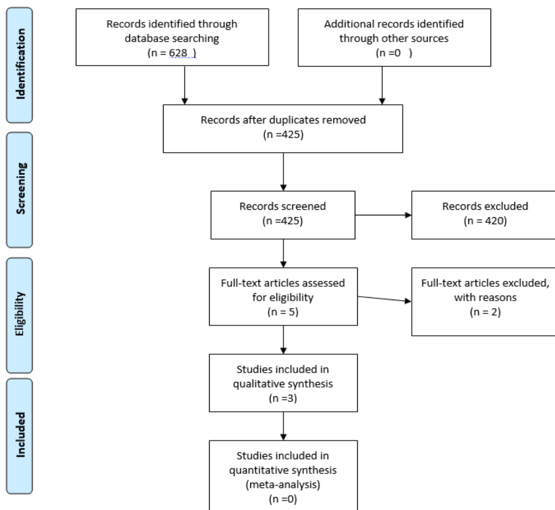
Fig.1: PRISMA flowchart.
